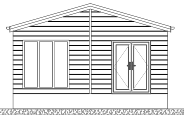
C Elevation
